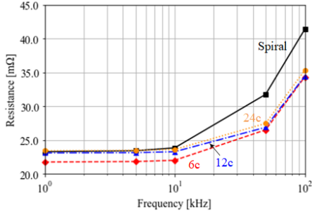
Fig. 3. FEM result of frequency characteristics of resistance
