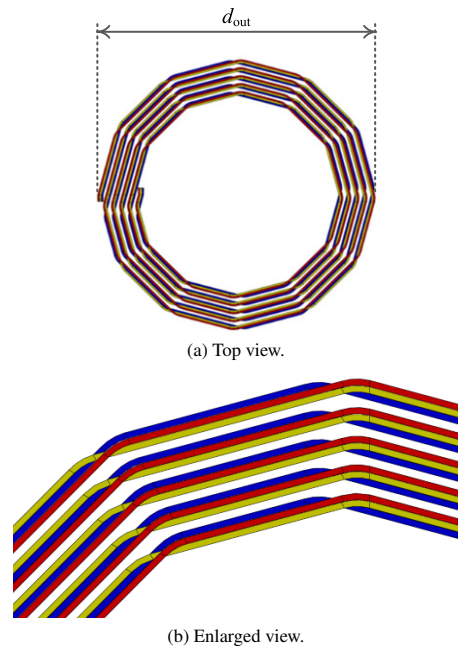
Fig. 1. Proposed coil structure
