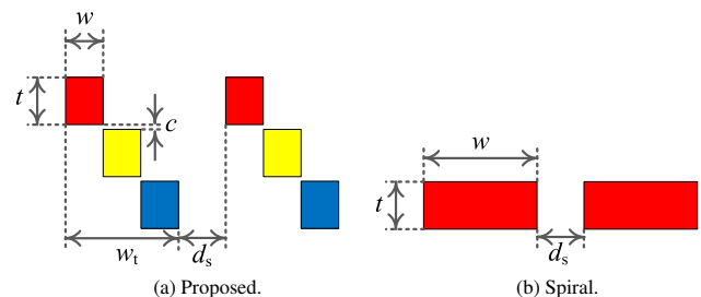
Fig. 2. The cross-sectional area of the spiral and proposed coils
